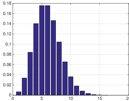
Figure 2: The Poisson distribution with \lambda = 5 .
